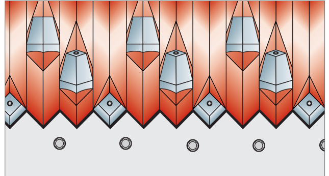
The V-rotor principle: optimum shredding results through precise cutting gaps.
